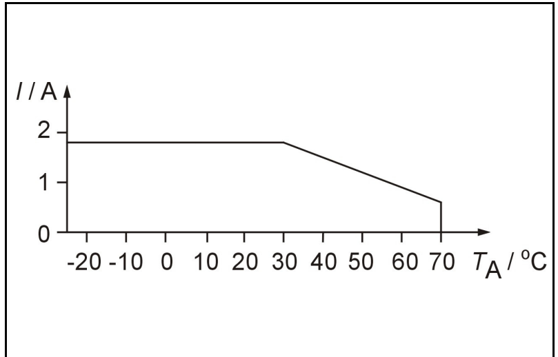
Derating curve for SLO 48CRA.
