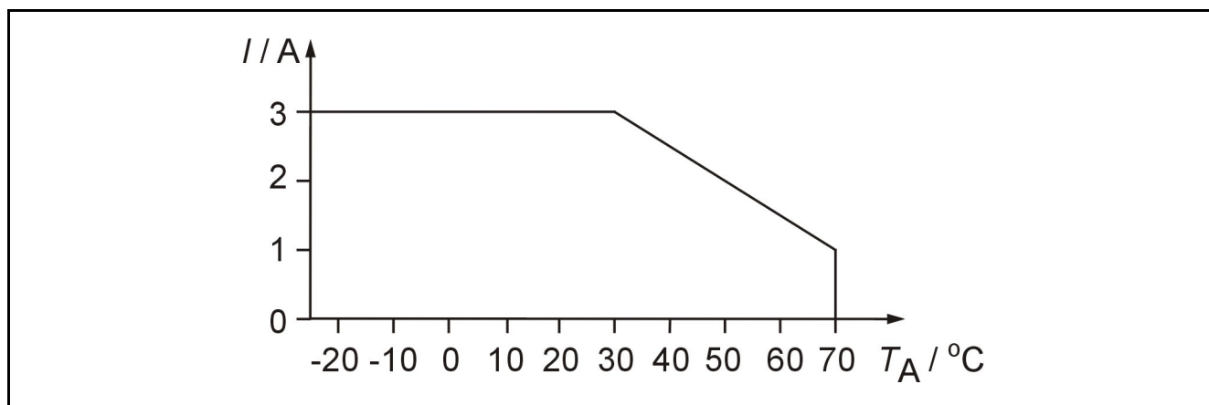
Derating curve for SLO 24CR.
