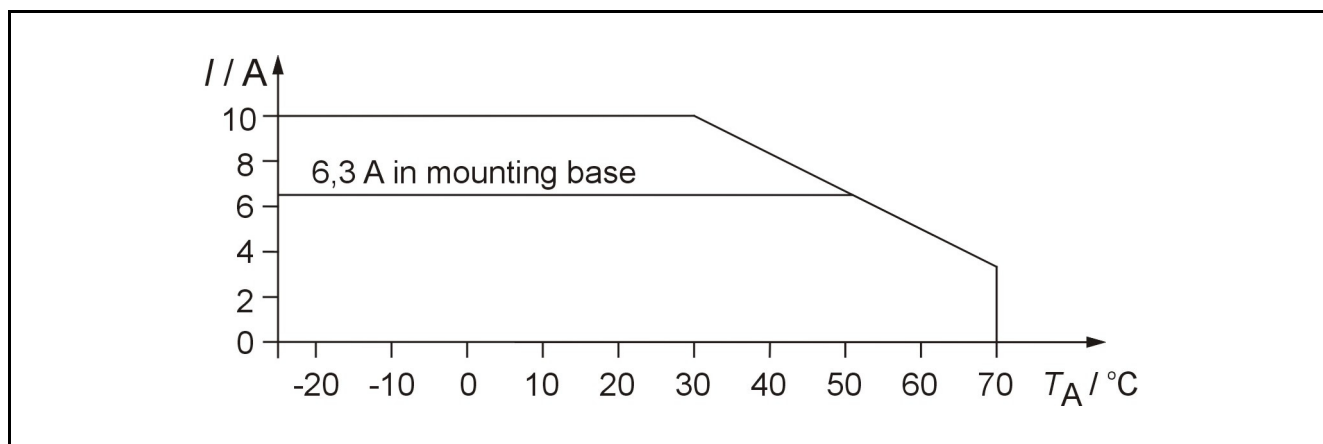
Derating curve for SLO 12CRX.
