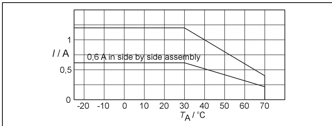
Derating curve for EXO 5IHA.
