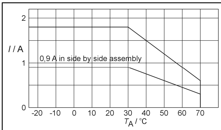
Derating curve for EXO 5CHA.
