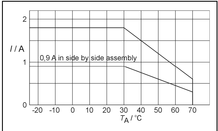
Derating curve for EXO 48CHA.
