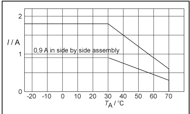
Derating curve for EXO 24CHA.
