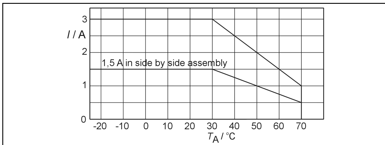
Derating curve for EXO 24CH.
