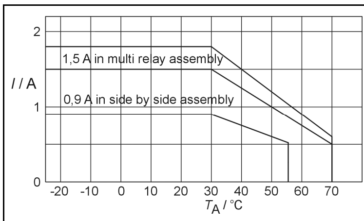
Derating curve for EXO 220CHA.
