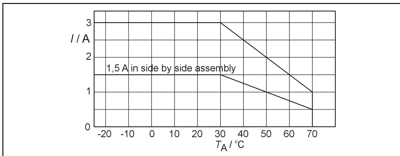
Derating curve for EXO 12CH.
