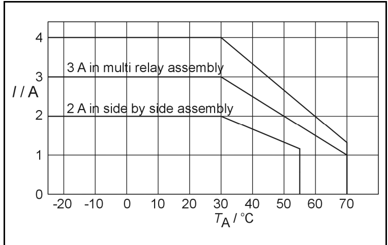
Derating curve for EXO 120CHA4.
