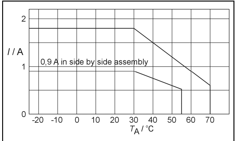
Derating curve for EXO 120CHA.
