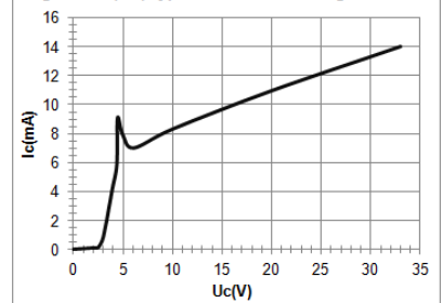
Fig.1 : I c =f(U c ) typ. , with mains voltage
