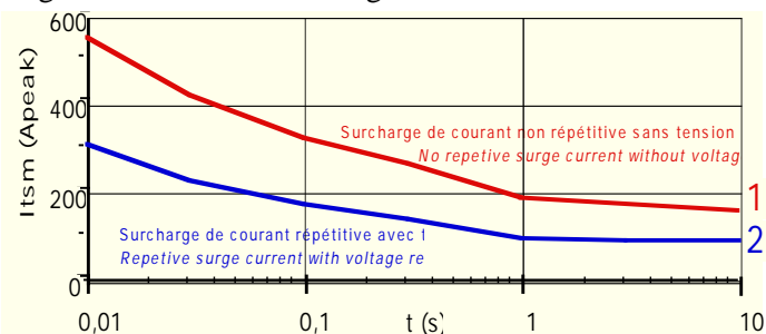
Fig 3 : Courants de surcharges/ Overload current
